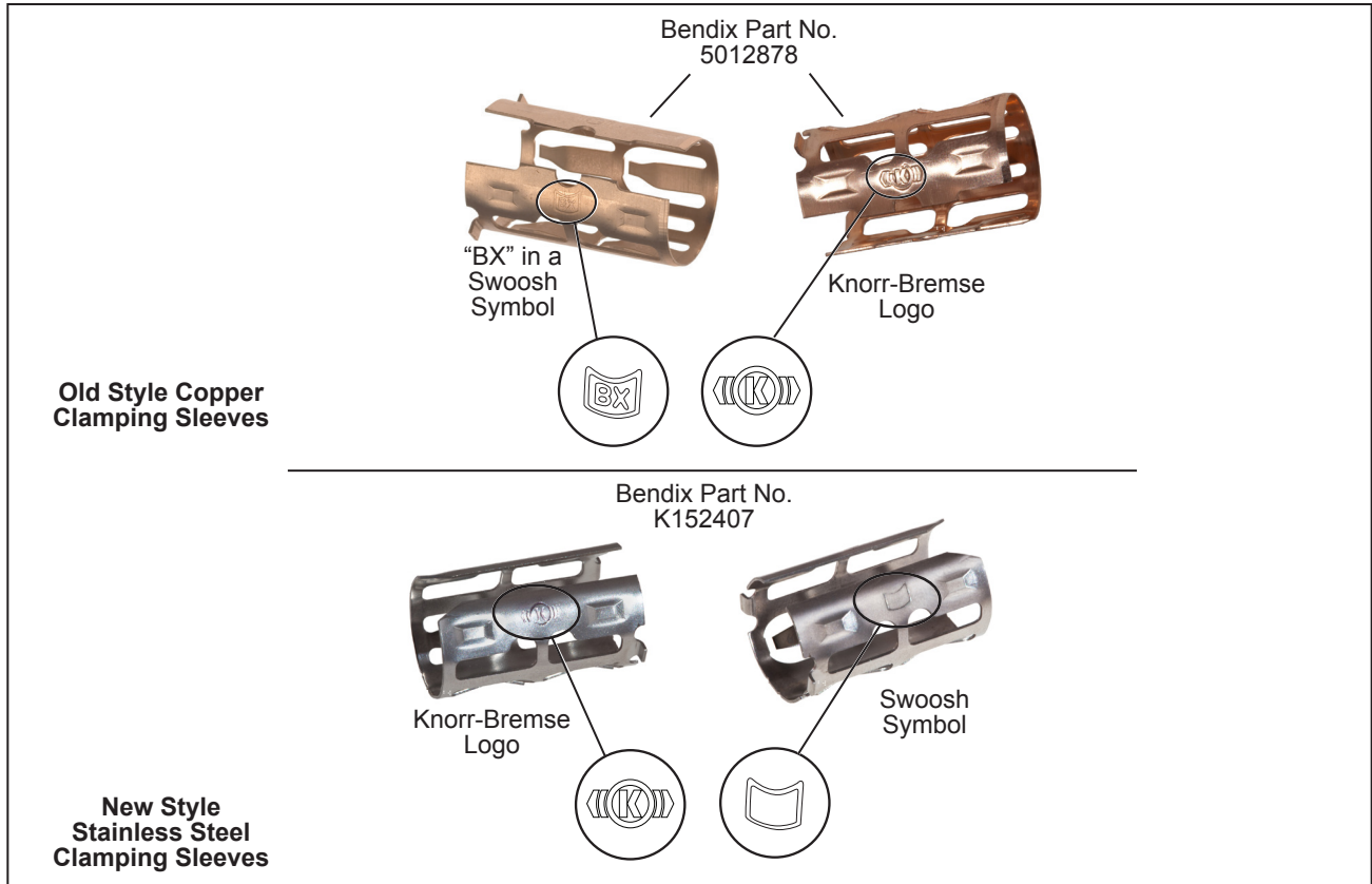
Figure 1 – Wheel Speed Sensor Clamping Sleeves
