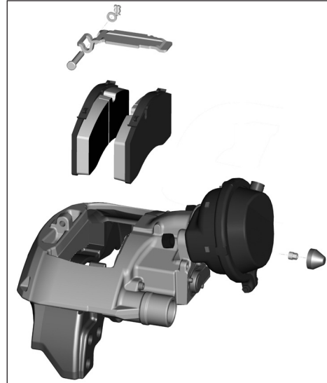
Bendix® ADB22X™ Pad Replacement Kit: Includes pads, pad retainer bar, bolt, washer, split pin, adapter and cap.
