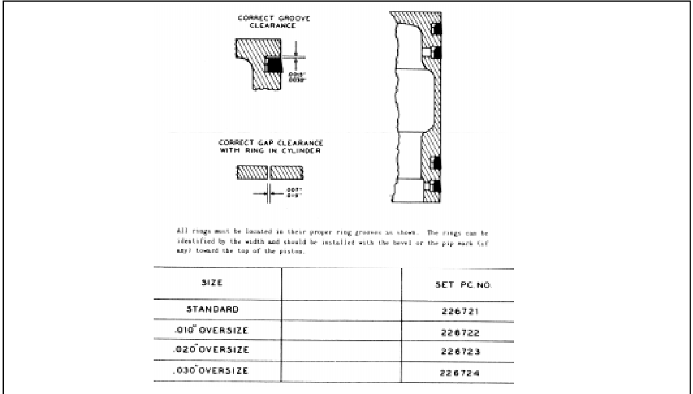
Figure 1 Tu - Flo 400 Compressor Rings
