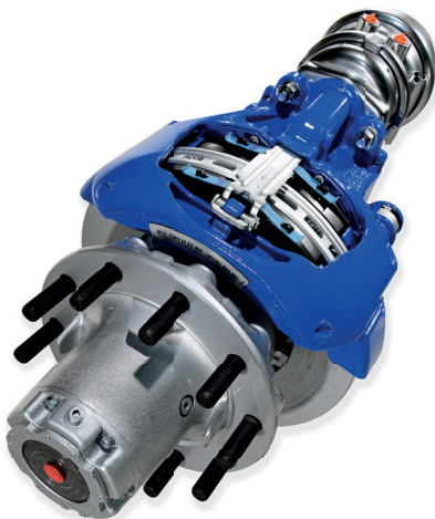
Bendix® ADB22X® and ADB22X®-LT for Tractor and Trailer
