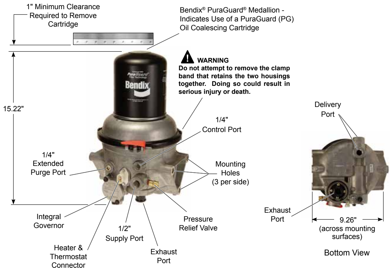
Bendix® AD-9si™ Air Dryer
