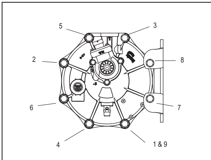
Figure 2 End Cover Bolt Torque Pattern
