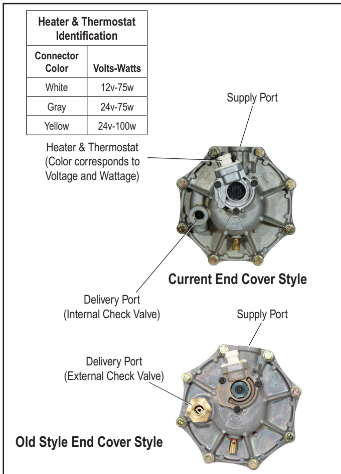
Figure 4 Bendix® AD-9® Air Dryer End Covers
