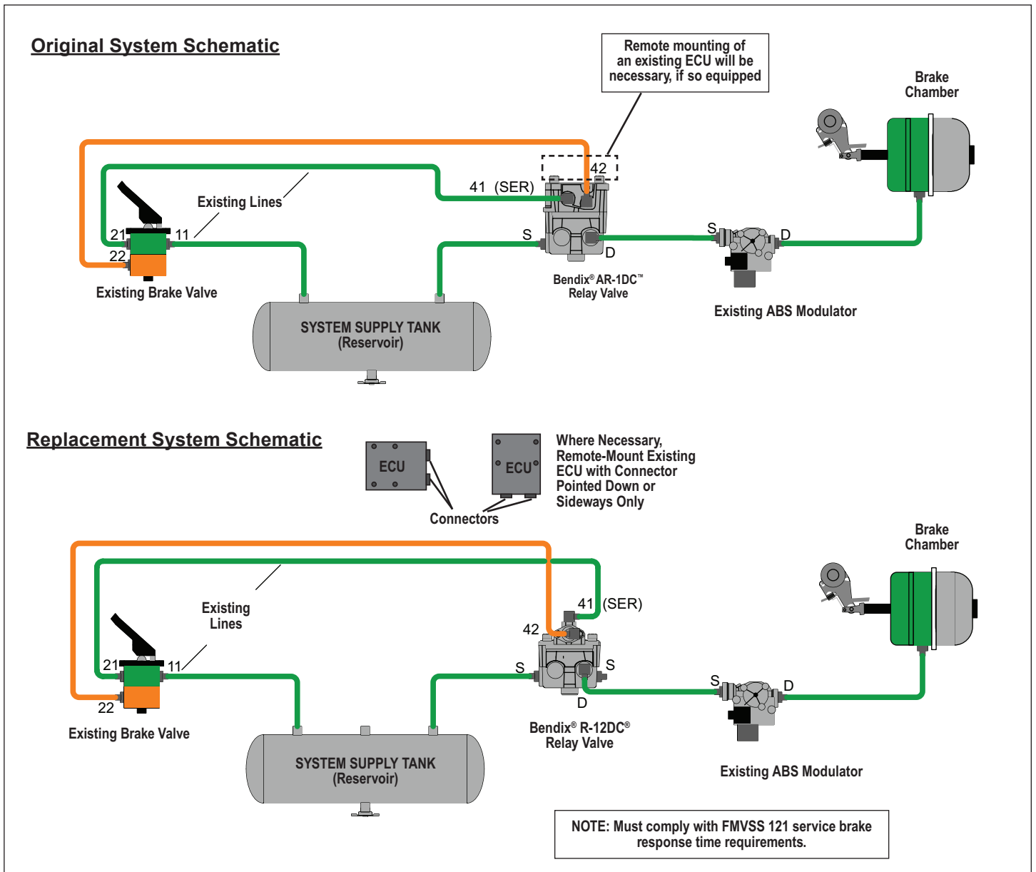
FIGURE 2 - SYSTEM SCHEMATICS
