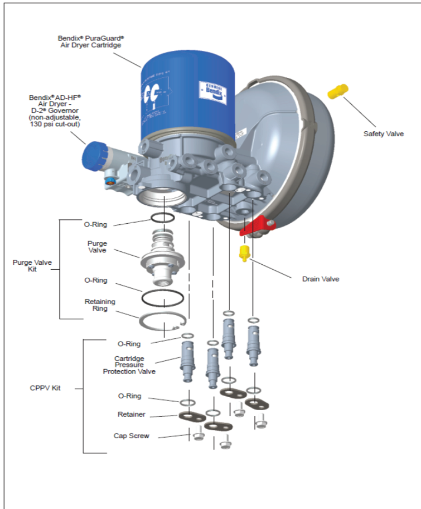
Cartridge Pressure Protection Valve (CPPV) Kit
