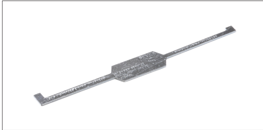
Figure 1 – Obsoleted Bendix® ES™ (Extended Service) Brake Lining Wear Gauge (PN 975465)
