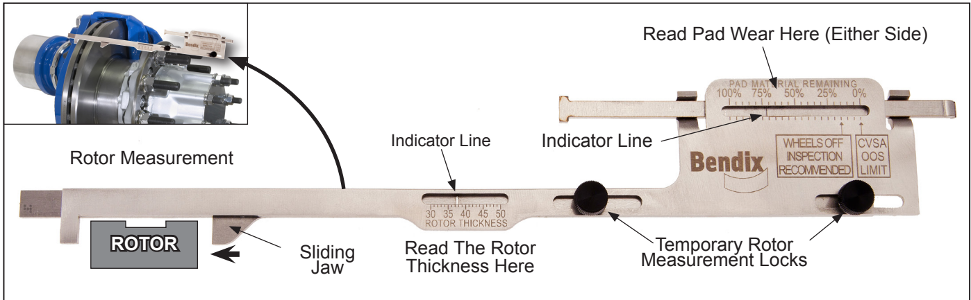
Figure 1 – Pad & Rotor Wear Gauge Tool
