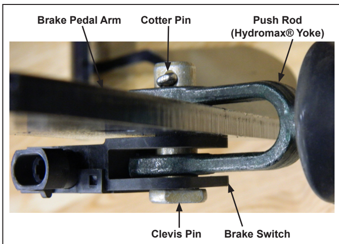
Figure 1 – Brake Pedal Components
