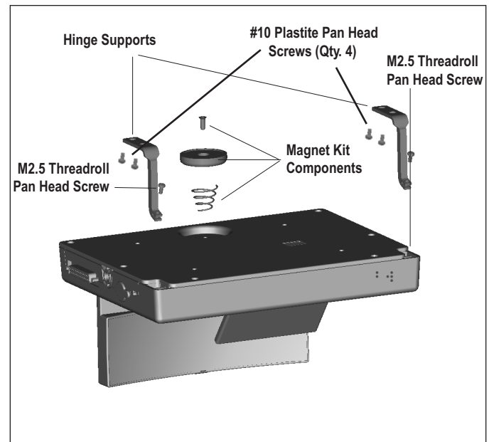
FIGURE 7 - FRICTION HINGE MOUNTING KIT COMPONENTS
