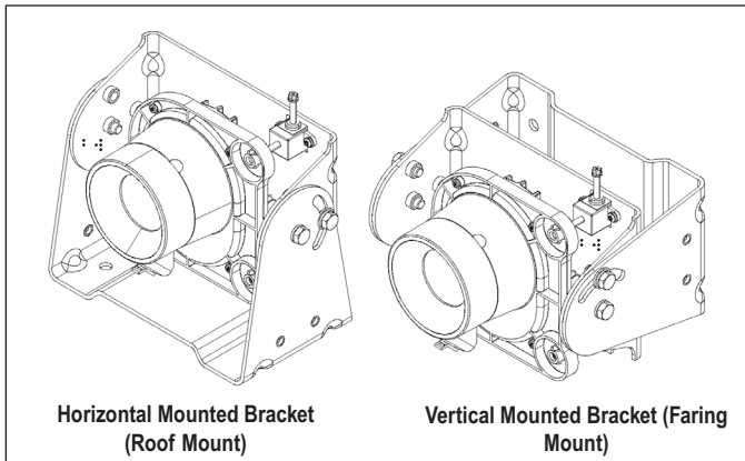
FIGURE 2 - MOUNTING BRACKET ORIENTATIONS
