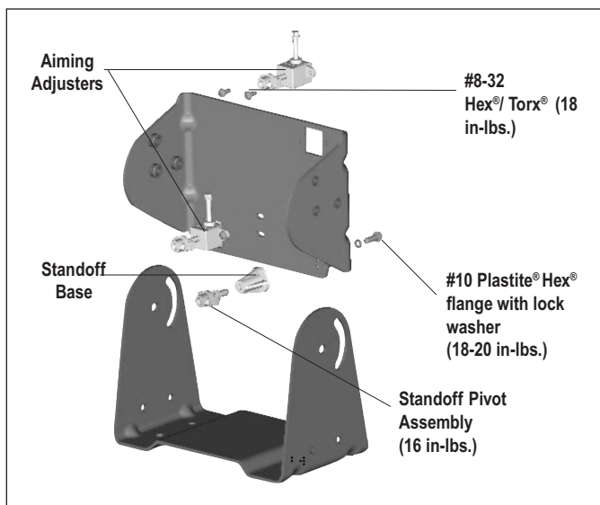
FIGURE 15 - AIMING ADJUSTER REPLACEMENT KIT
