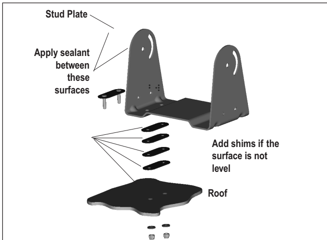
FIGURE 3 - MOUNTING BRACKET KIT CONTENTS
