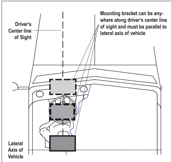
FIGURE 20 - MOUNTING BRACKET AND LATERAL AXIS OF VEHICLE
