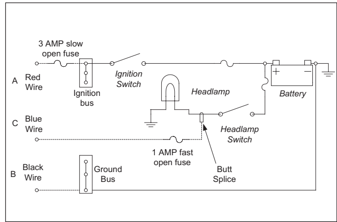
FIGURE 34 - XVISION SYSTEM ELECTRICAL POWER SCHEMATIC
