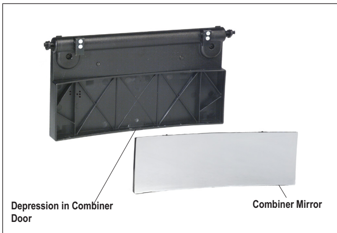
FIGURE 28 - REPLACEMENT COMBINER
