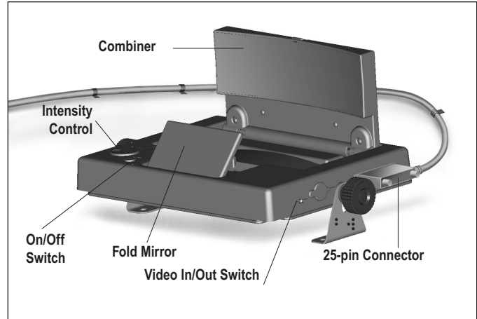
FIGURE 13 - DISPLAY (SHOWN IN CB STYLE MOUNT (DASHBOARD) POSITION WITH DISPLAY HARNESS)
