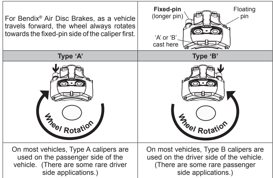
FIGURE 1 - TYPE 'A' AND 'B' BRAKES
