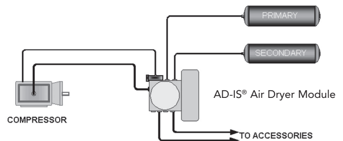
Bendix® AD-IS® air dryer module system schematic
