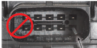
Bent/Broken/Missing Terminals
