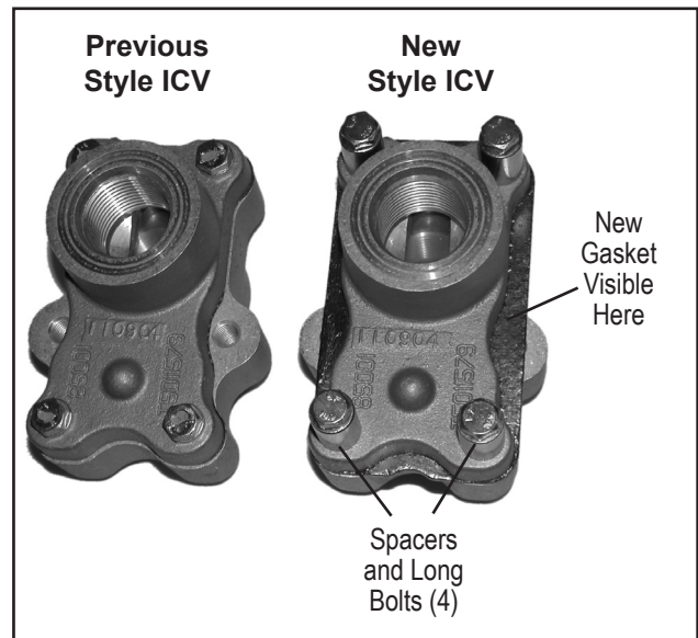
FIGURE 1 - Comparison Showing New Gasket
