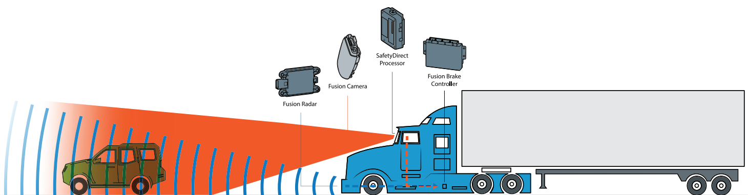
Figure A Bendix Fusion integrates complementary systems – the radar, camera, and brakes, plus the SafetyDirect web portal – to help provide enhanced safety for today's North American commercial vehicles.
